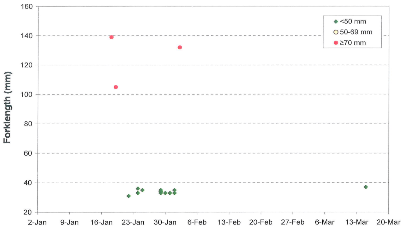
2010 Grayson screw trap salmon
