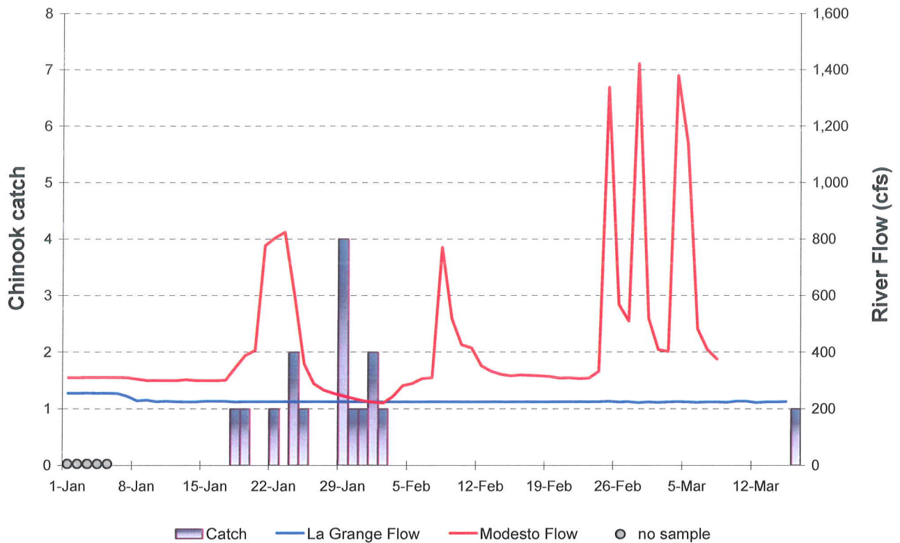
2010 Grayson screw trap salmon
