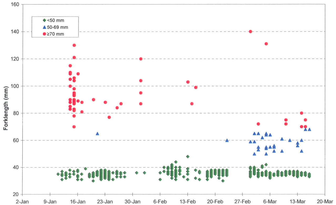
2010 Waterford screw trap salmon
