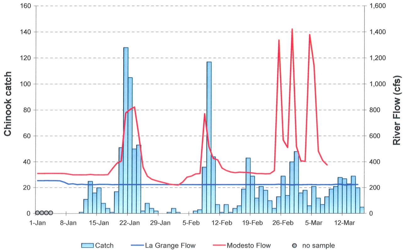
2010 Waterford screw trap salmon
