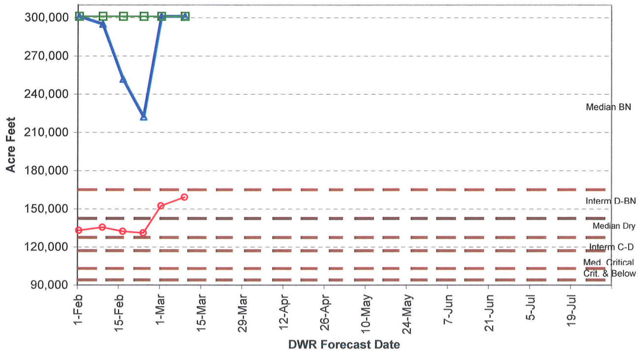
2010-2011 FERC Flow Volumes (10%, 50% 90% exceedence values)
