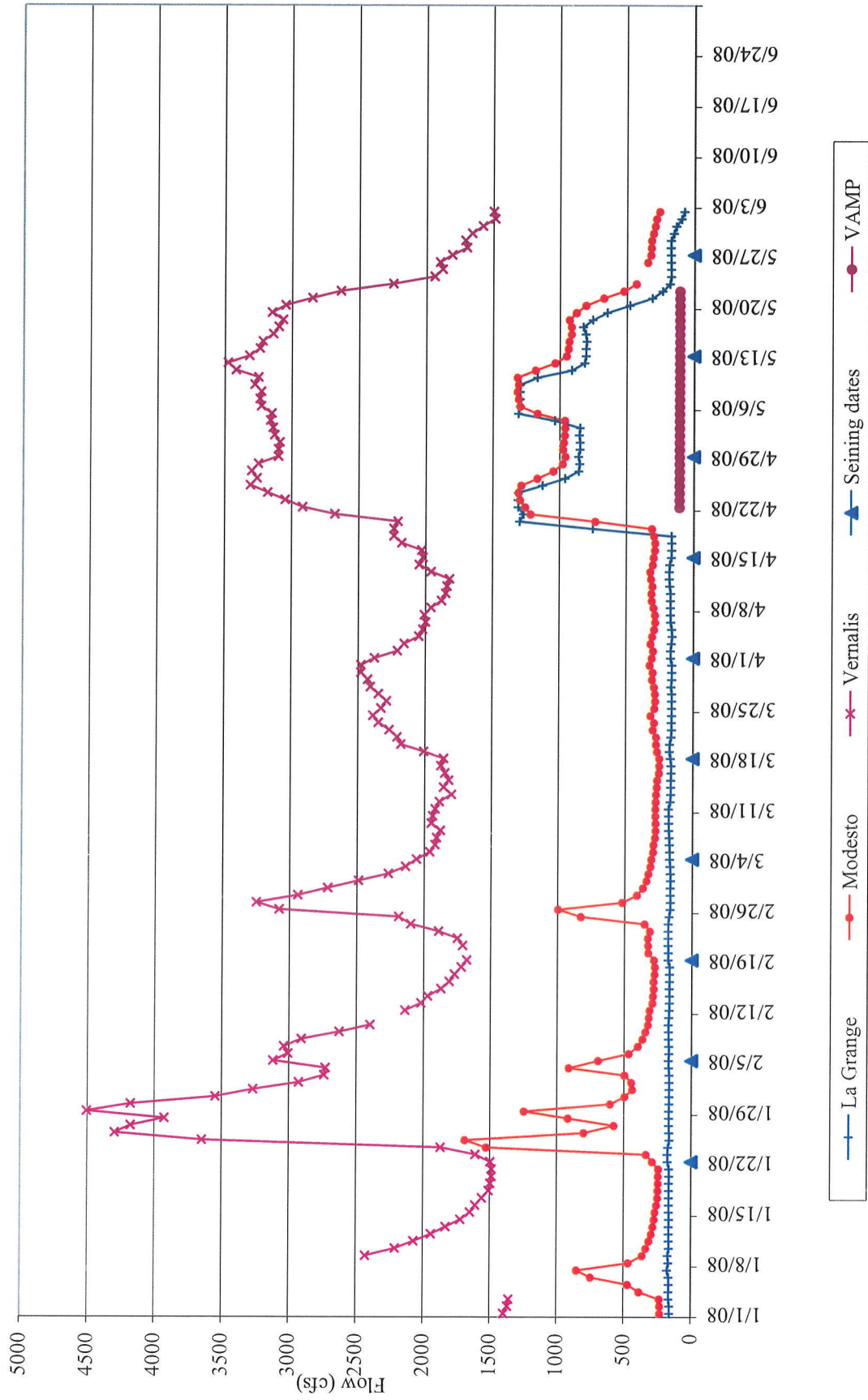
2008 Tuolumne and San Joaquin River daily mean flow Provisional USGS data
