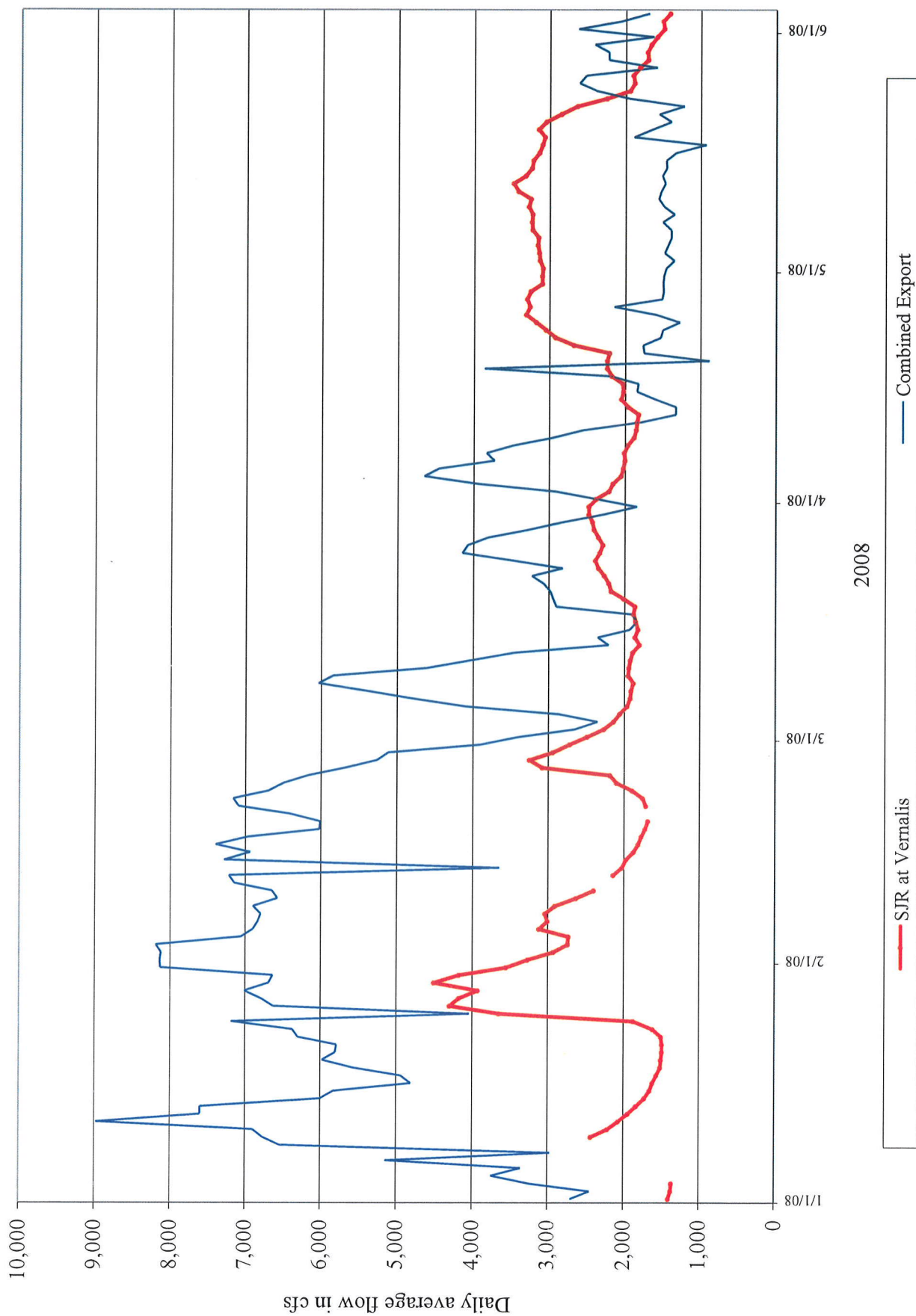
Daily average flow at Vernalis (SJR) and combined CVP and SWP delta export
