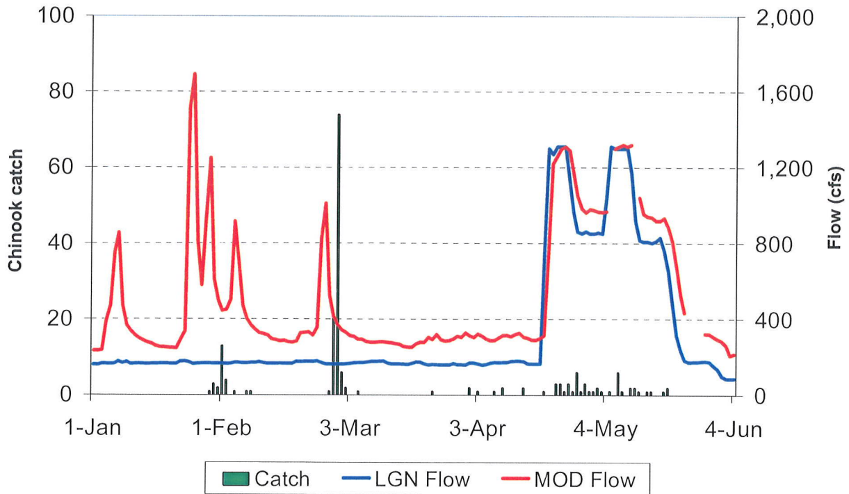
2008 Chinook Catch at Grayson and Tuolumne River Flow at La Grange and Modesto
