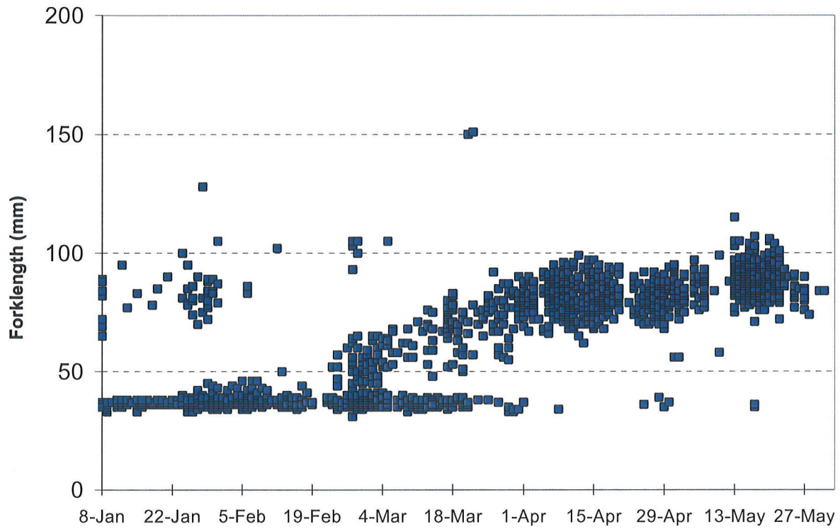
Lengths of Chinook Captured at Waterford - 2008
