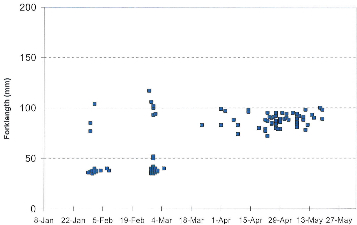
Lengths of Chinook Captured at Grayson - 2008
