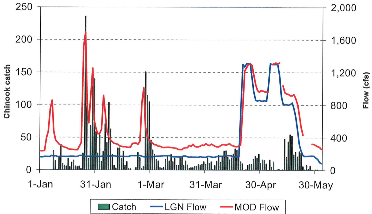
2008 Chinook Catch at Waterford and Tuolumne River Flow at La Grange and Modesto
